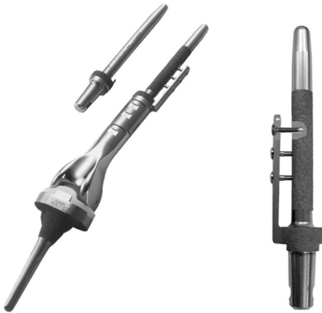
Fig. 1 The detailed features of the KMLS system. Left Cement-type femoral stem and cementless-type femoral stem and prosthesis. Right Three unique partial-holes and a side plate with three screw holes of the cementless-type femoral stem component
